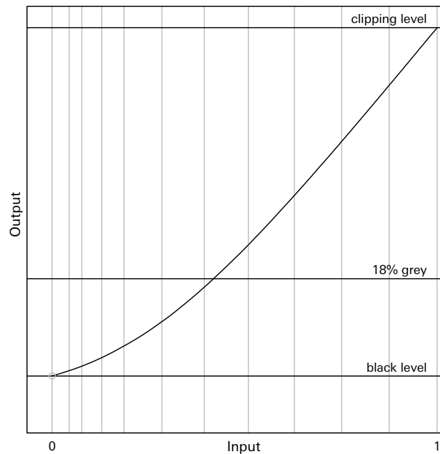
LOG F characteristic curve
