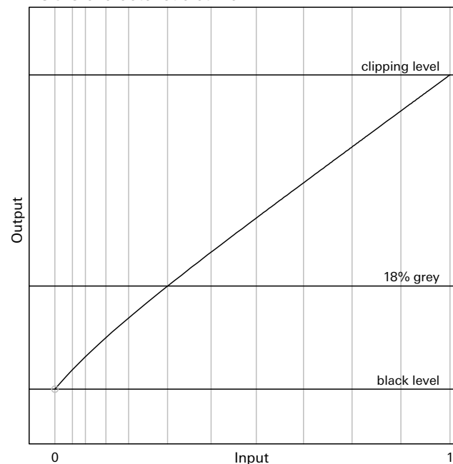
LOG C characteristic curve
