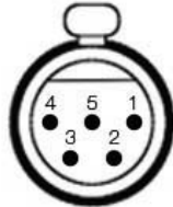
Line Audio Output Signals (5-pin mini-XLR) Connector
